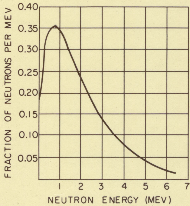
Figure 2. Fission neutron energy distribution Murray (11, p. 57)
